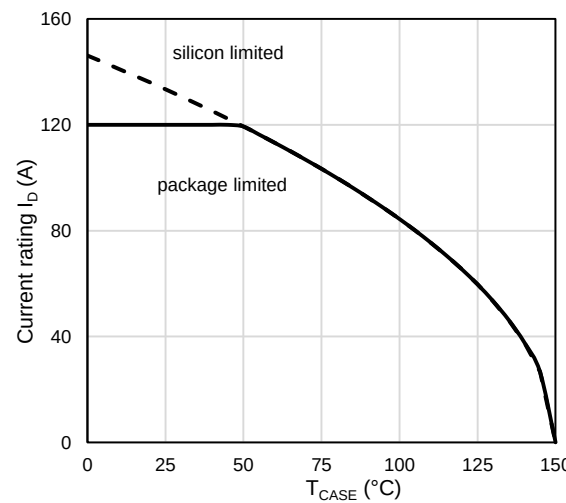
Figure 12: Current De-rating
